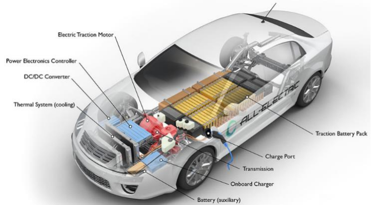
Figure 17 BEV Major Components
