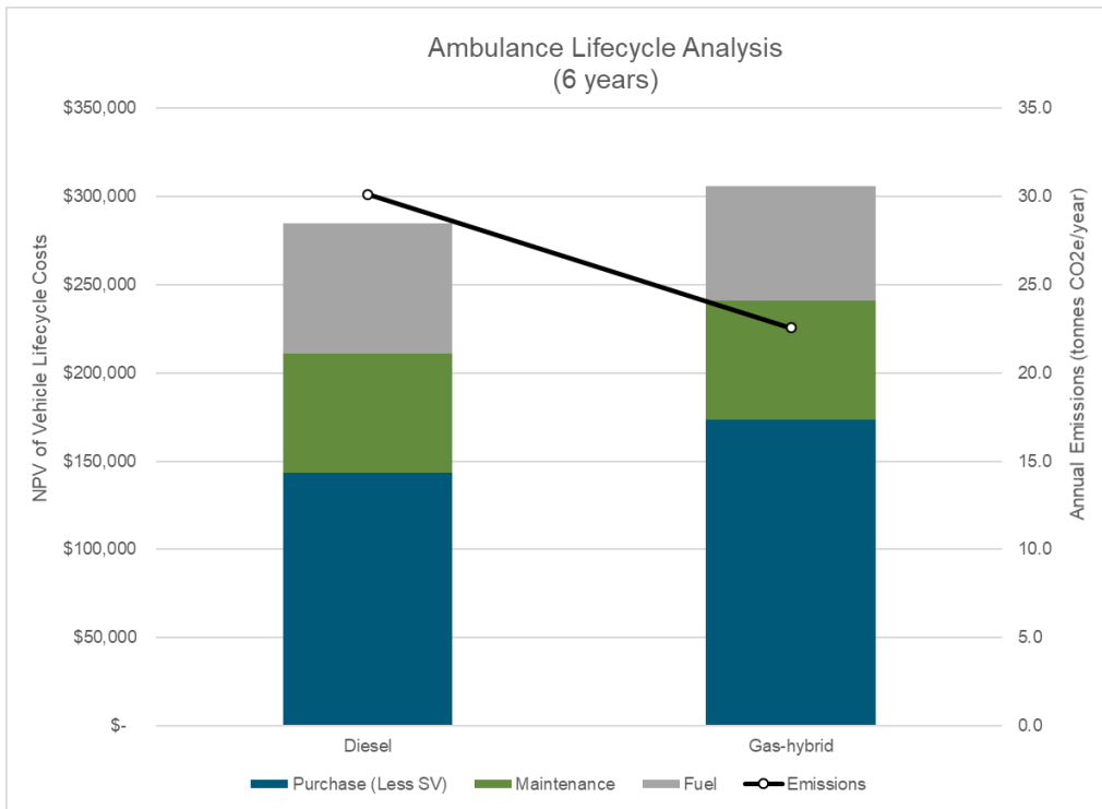
Figure 43 Ambulance Lifecycle Analysis
