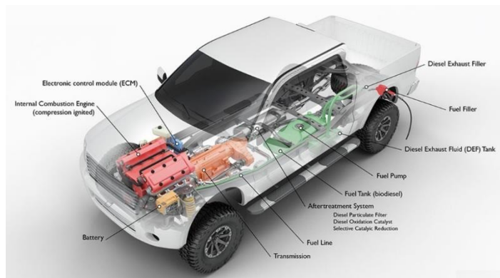
Figure 12 Bio-diesel Vehicle Components
