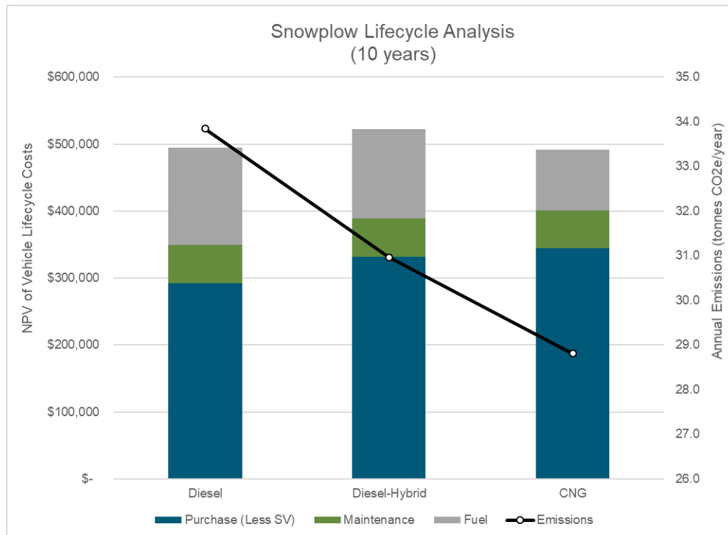
Figure 38 Snowplow Lifecycle Analysis
